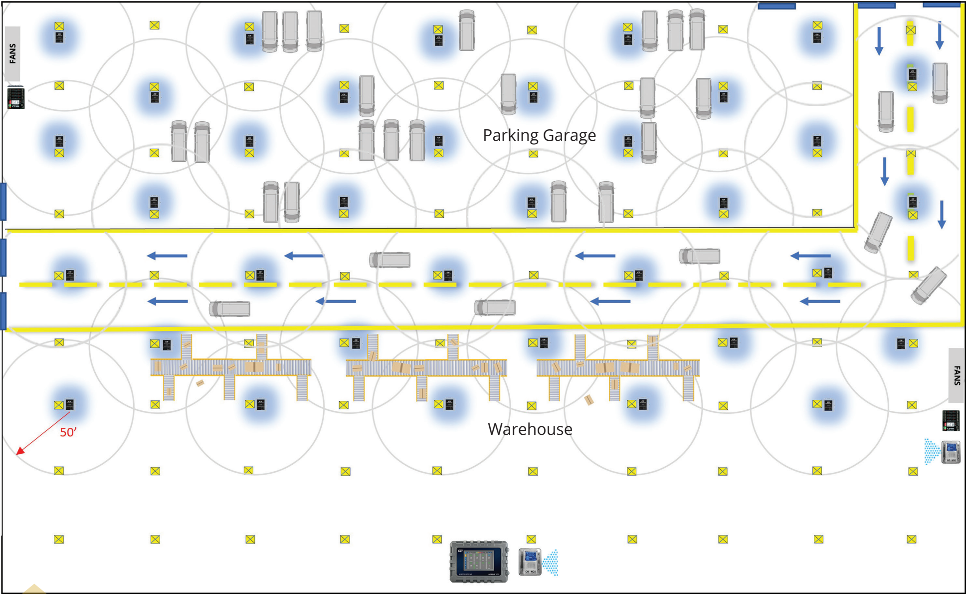
CTI's System Layout Sensors placed on every other support column and concentrated in areas containing vehicles and personnel.
