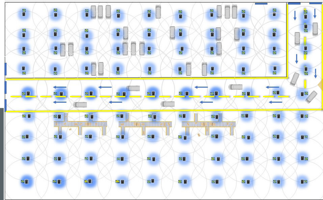
Competitor's System Layout Sensors placed on every support column creating unnecessary overlap and inflated initial installation and ongoing maintenance costs.
