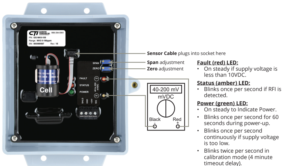
Figure 3: Sensor board components and zero/span adjustment
