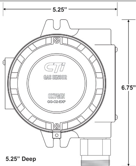
Figure 1: Mounting Dimensions
