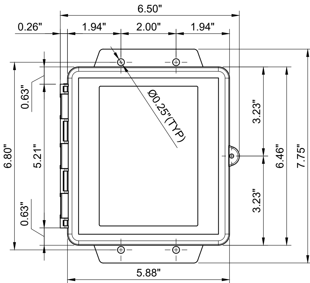
FRONT VIEW
