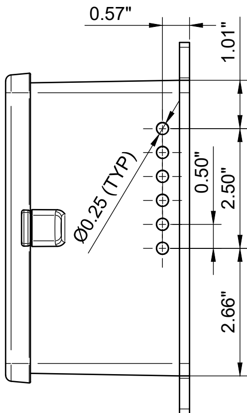
RIGHT VIEW
