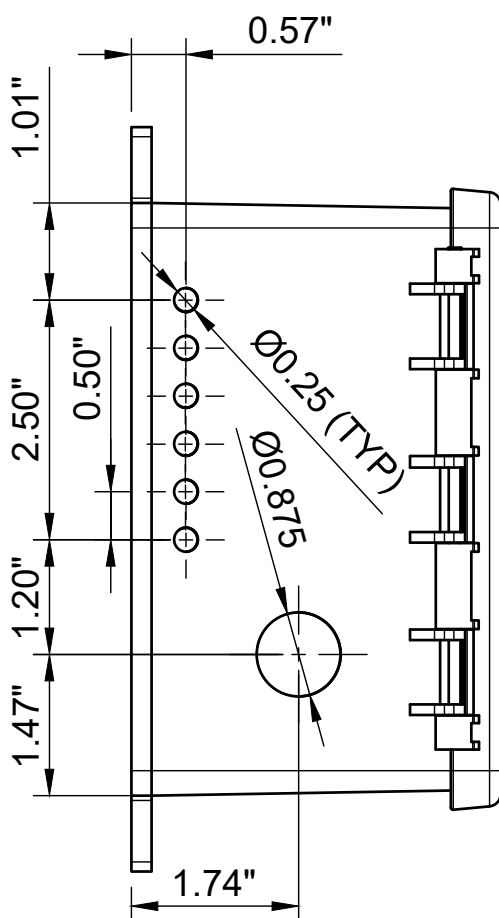
LEFT VIEW
