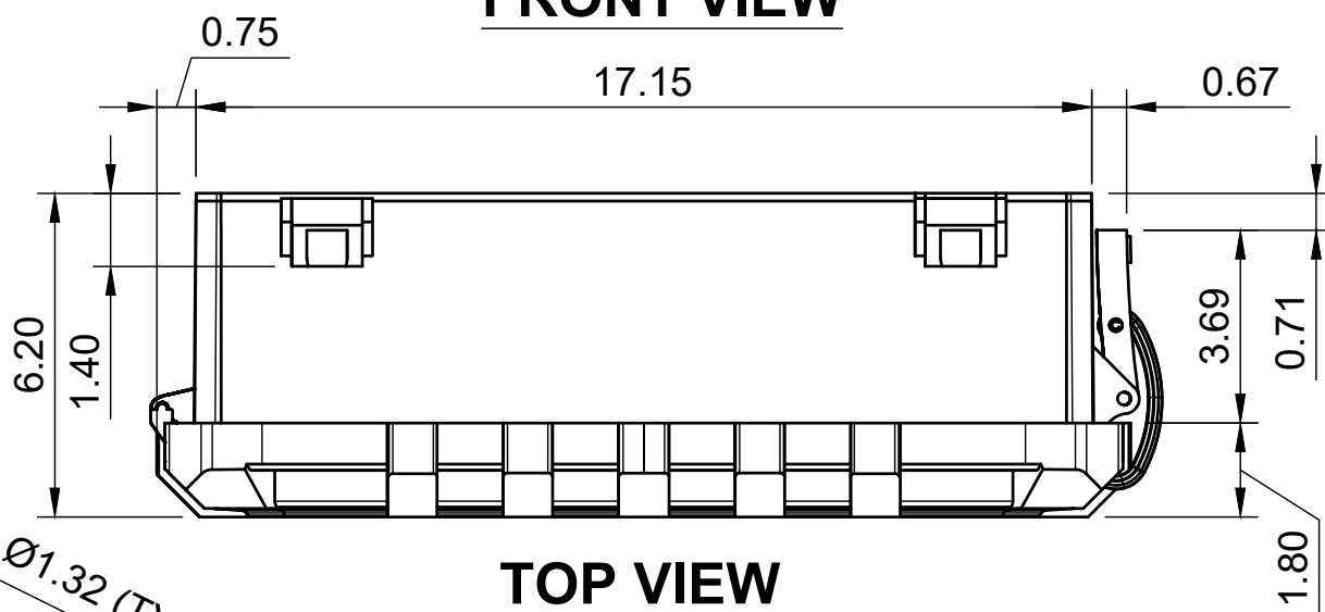
FRONT VIEW
