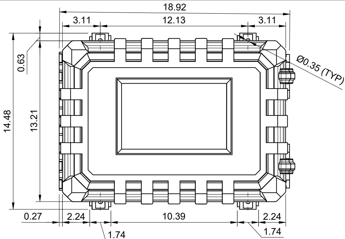
FRONT VIEW
